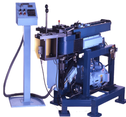
S1060 Rotary Draw Bender
