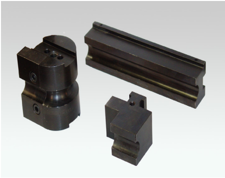
Bend Tooling designed and built for Lomar Benders and competitors.
